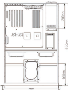
Zippy MRG Series 200mm deep RPS
