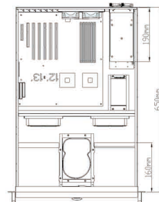
FSP RRP4ATX6508 Series 190mm deep RPS
