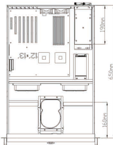
Etasis EFRP Series 190mm deep RPS
