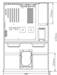
Enermax EMA Series 199mm deep RPS
