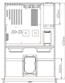
Zippy MRT/MRW Series Enhance ENR Series 185mm deep RPS
